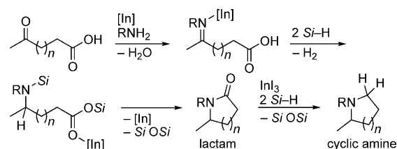
Scheme 6. A plausible mechanism.
